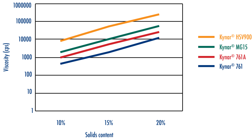
Figure 3: Kynar® solution viscosity in NMP 25°C @ 10s -1
