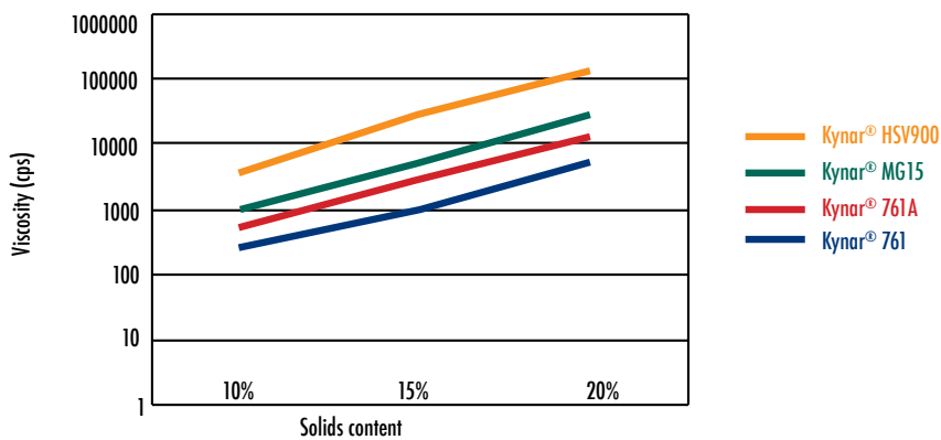
Figure 4: Kynar® PVDF solution viscosity in DMAc, 25°C @ 10s -1
